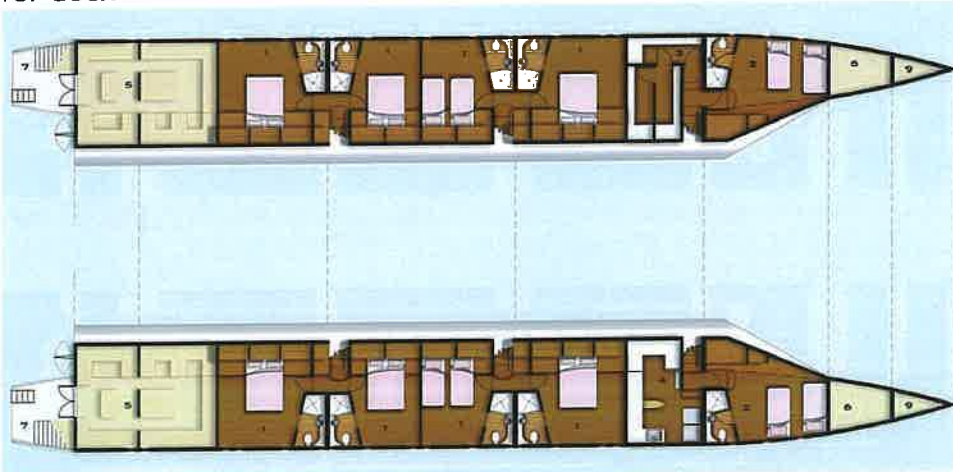
main deck
